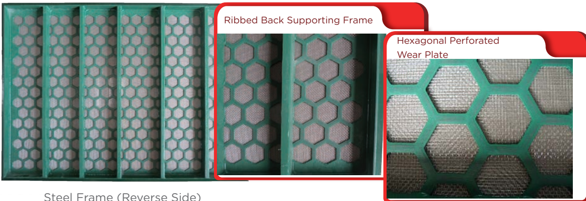
Steel Frame (Reverse Side)
